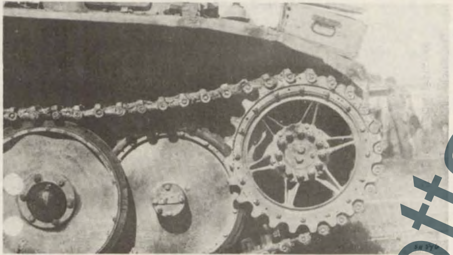
Close-up view of front driving sprocket.
